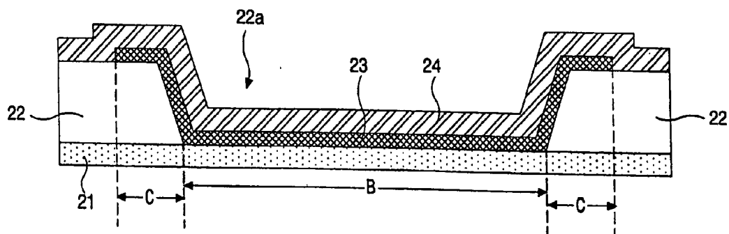
FIG. 3 Related Art
